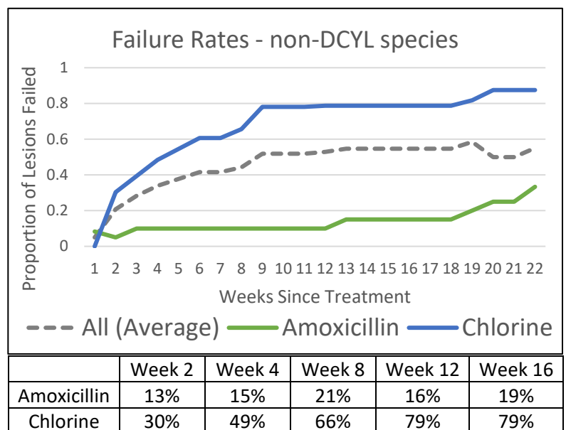
Figure 1: Proportional failure rates of amoxicillin and chlorine treatments in non- D. cylindrus species
