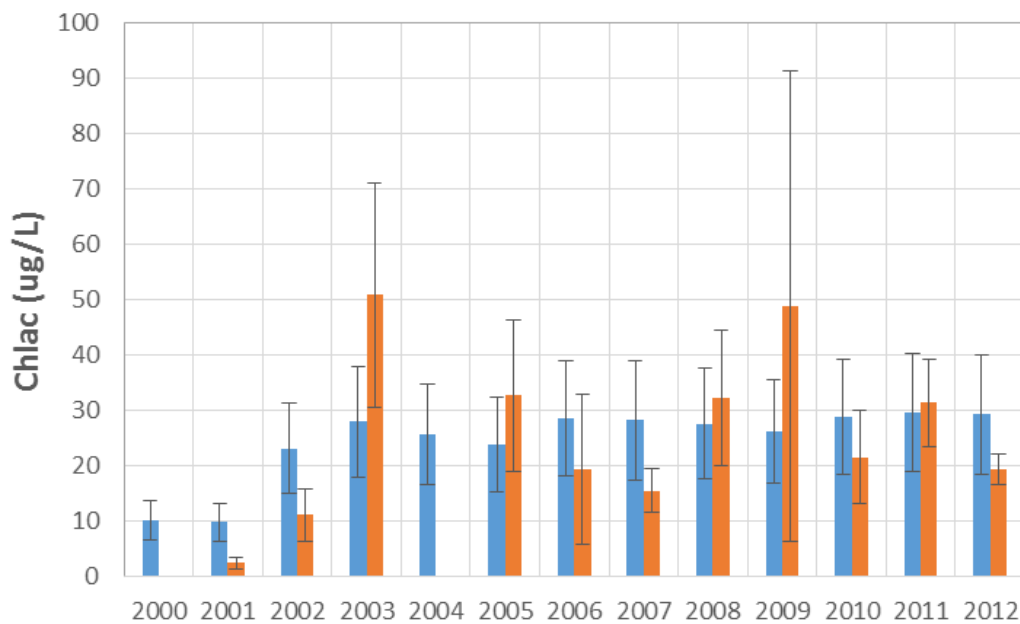
Figure 5.16. Calibration of simulated annual Chla (blue bars) with observed annual Chla (orange bars) in Lake Roberts, 2000–12
