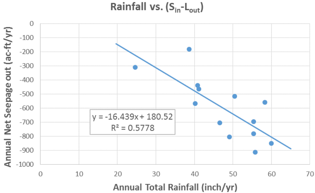
Figure 5.10. Relationship between annual total rainfall versus the sum of annual seepage-inflow minus annual lake outflow ( S_{in} - L_{out} ), 2000–12
