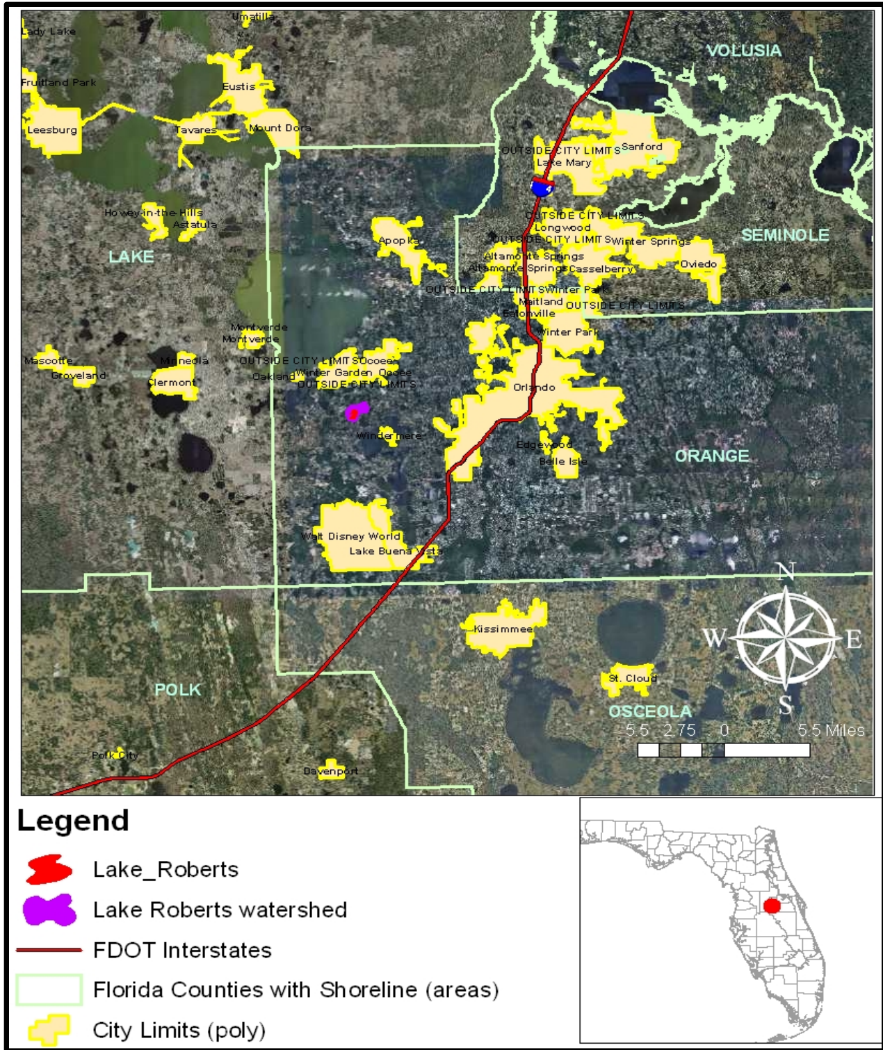
Figure 1.1. Geographic location of Lake Roberts in central Florida and major geophysical features in the area
