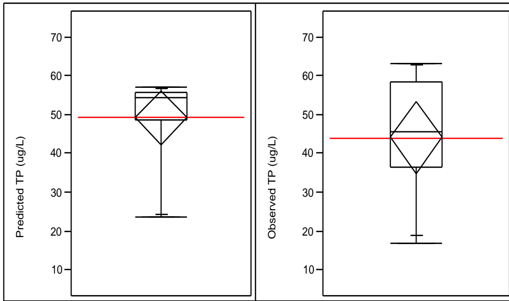
Figure 5.13. Box and whisker plot of simulated versus observed TP in Lake Roberts. The red line and diamond represent a long-term mean with 95 % confidence levels.
