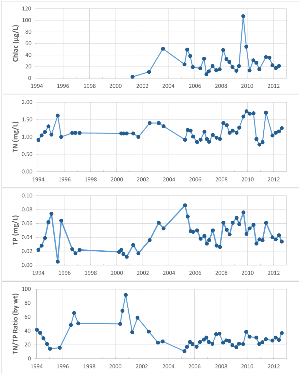
Figure 5.2. Long-term trend concentrations of Chl a, TN, and TP and TN/TP ratios in Lake Roberts, 1994–2012
