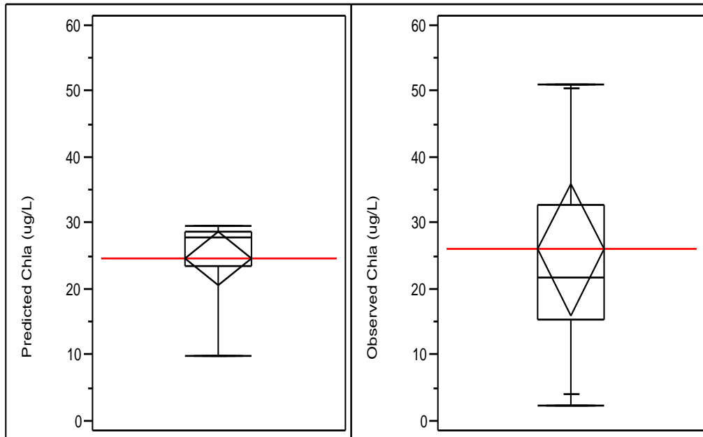
Figure 5.17. Box and whisker plot of simulated versus observed Chla in Lake Roberts. The red line and diamond represent a long-term mean with 95 % confidence levels.
