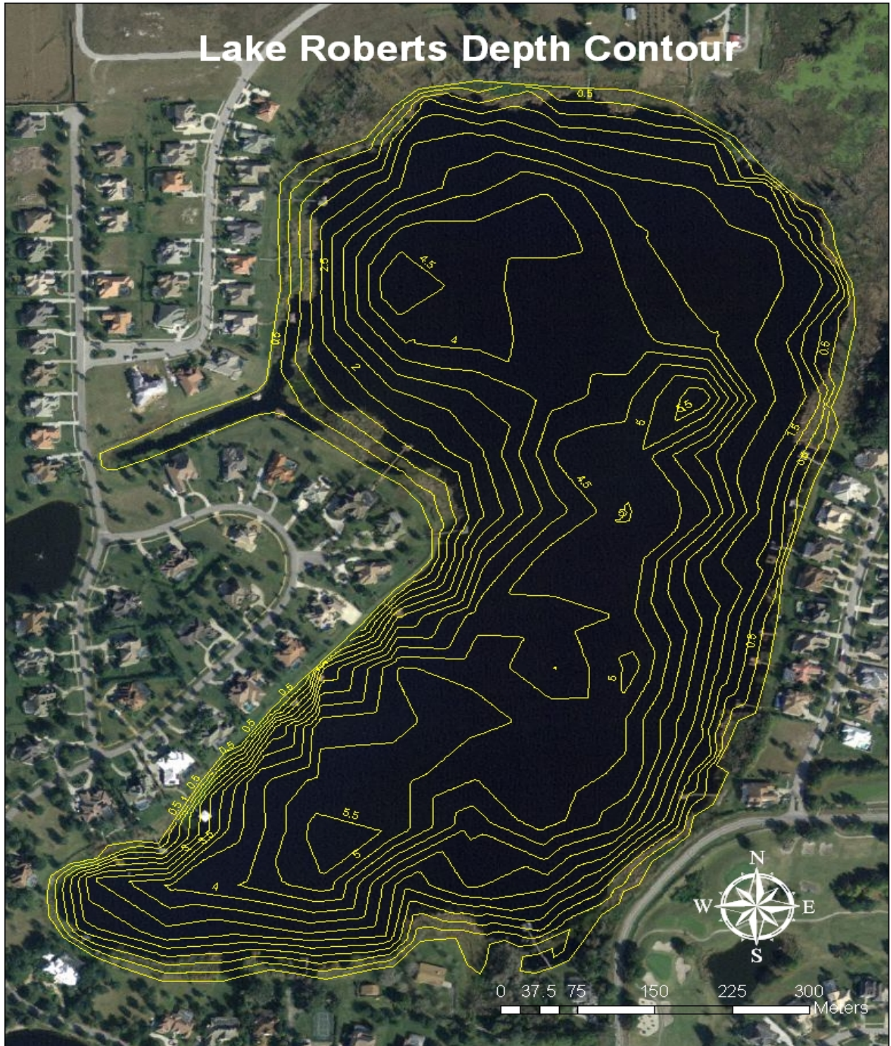
Figure 5.4. Bathymetric map generated for Lake Roberts using ArcGIS. Each contour line represents a 0.5-m depth interval.
