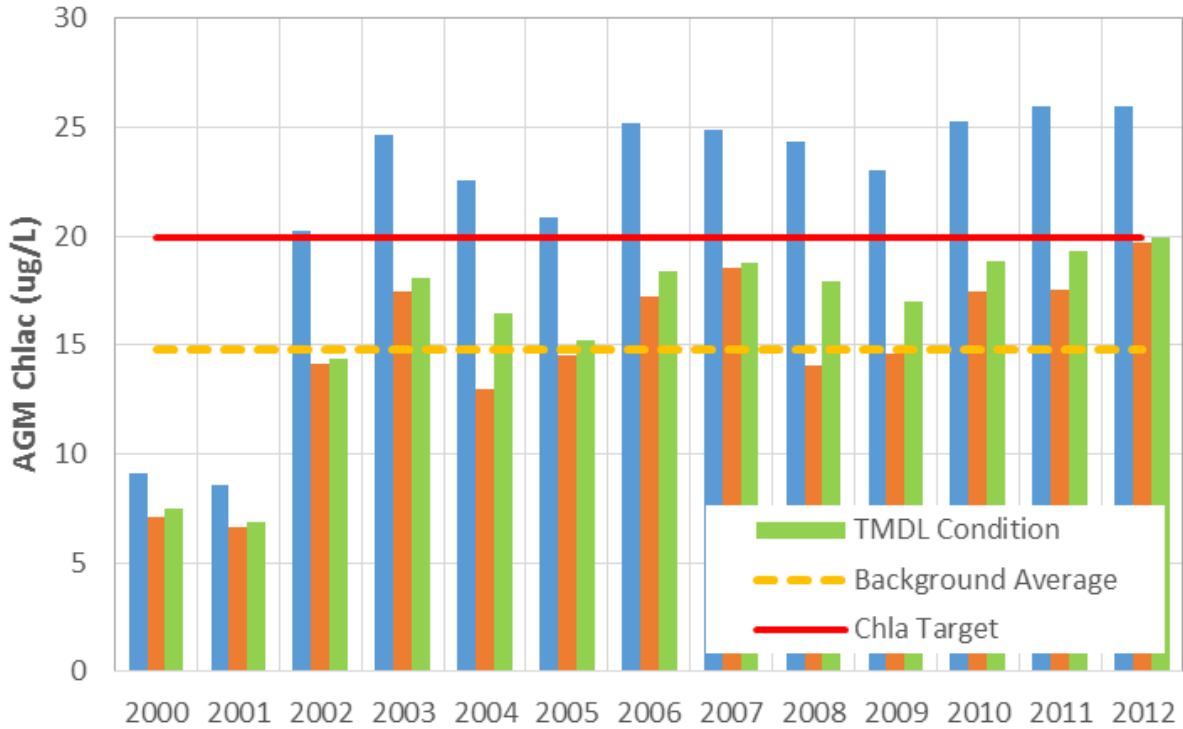
Figure 5.23. Simulated AGMs of Chla for existing (blue bars), natural background (orange bars), and TMDL conditions (green bars). The red line represents the Chla target of 20 µg/L for Lake Roberts.
