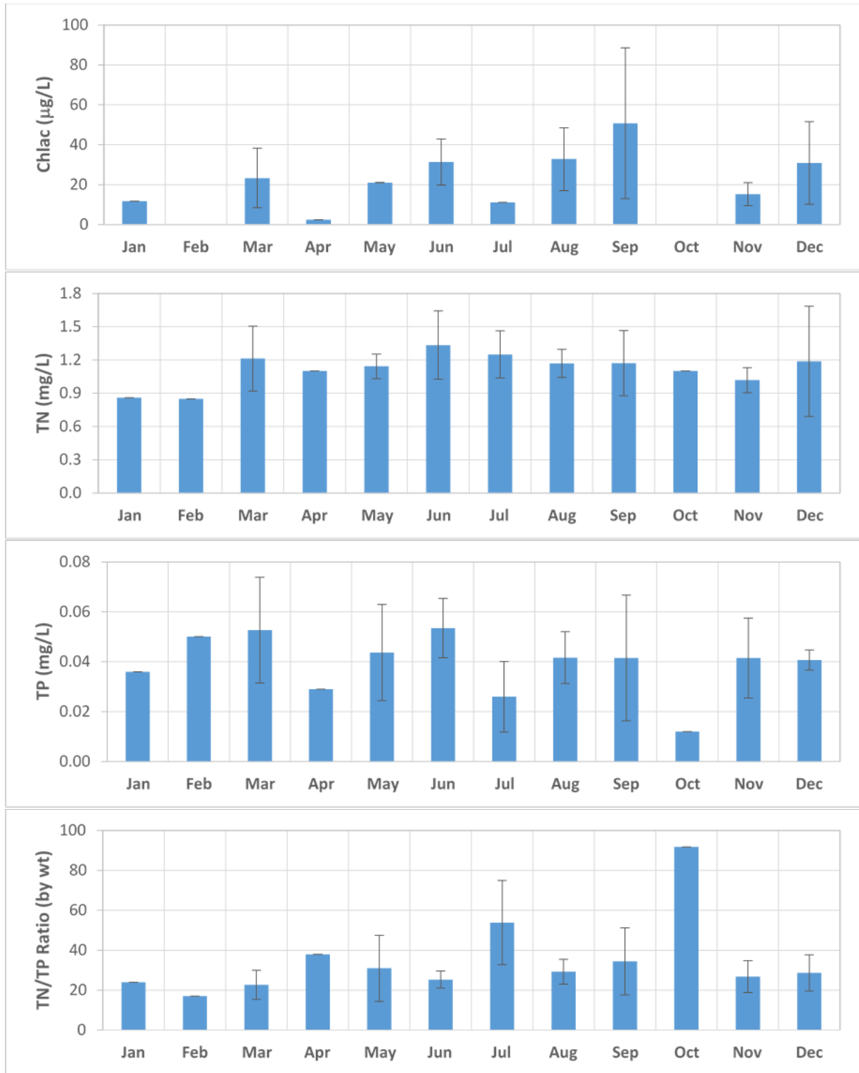
Figure 5.3. Monthly variations of Chl a, TN, and TP and TN/TP ratios in Lake Roberts, 2000–12. Error bars represent a 1-sigma standard deviation.
