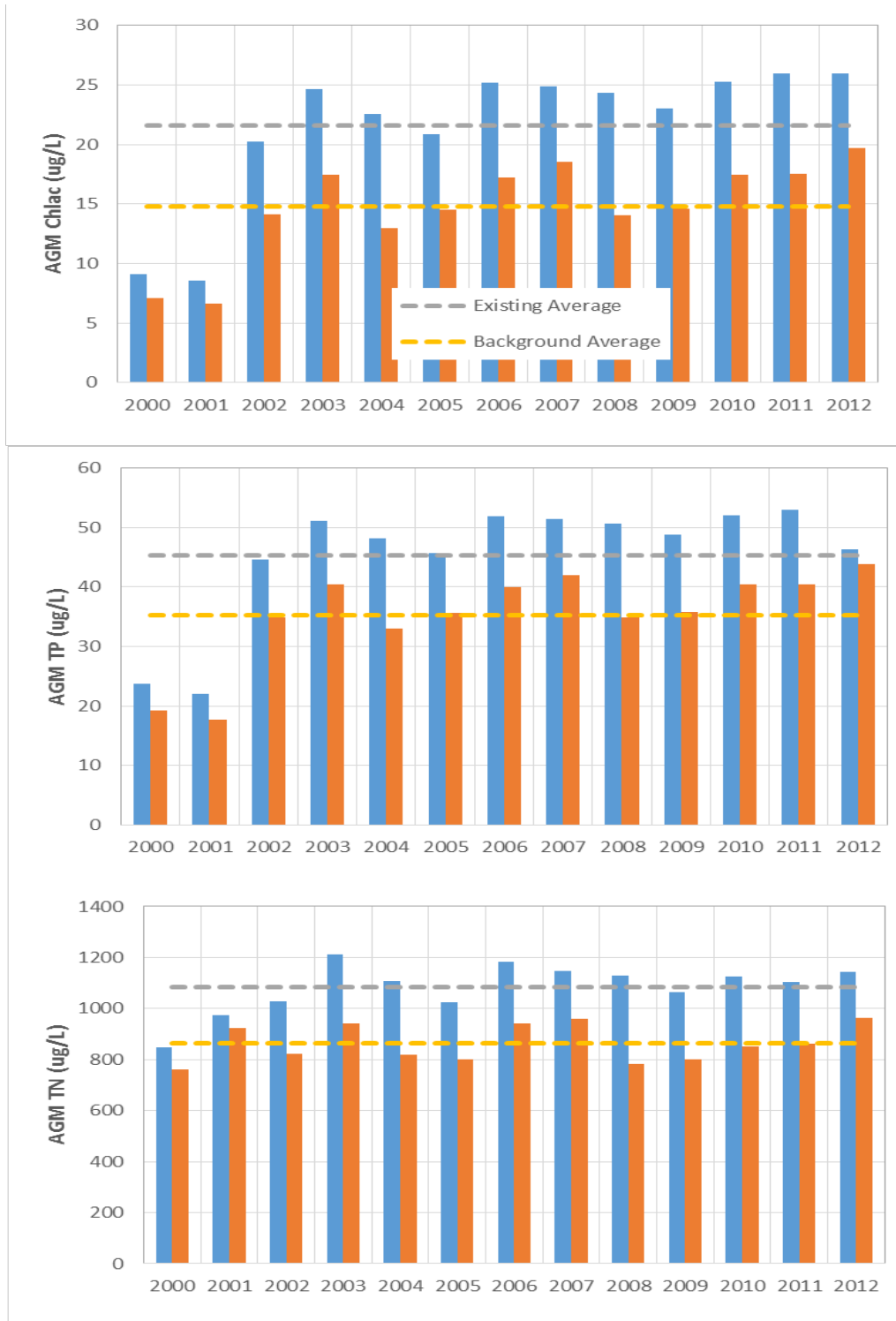
Figure 5.21. AGMs of Chla, TN, and TP for existing (blue bars) versus natural background (orange bars) conditions, 2000–12. Gray and yellow dashed lines represent the long-term averages of existing and natural background conditions, respectively.
