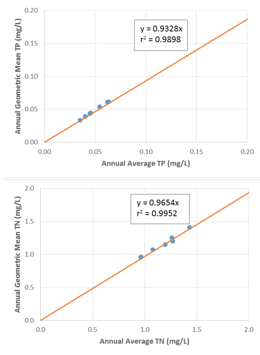
Figure 5.20. Linear relationships between AGMs and annual average concentrations of TP (top) and TN (bottom) used for lake NNC development. The dataset (circles) obtained from the observed data for Lake Roberts were plotted along the regression lines derived from the lake NNC dataset.
