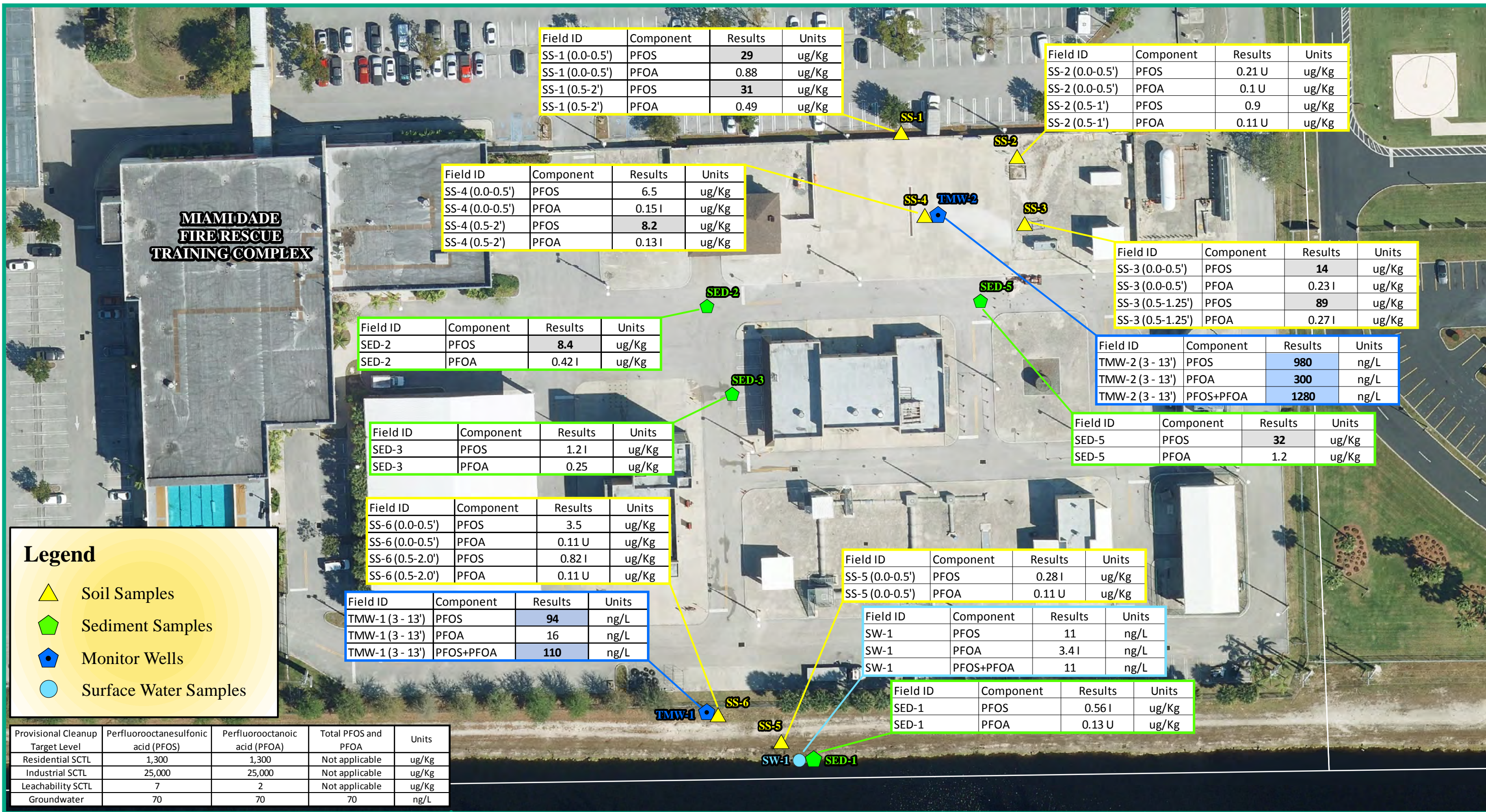
Figure 2 Sample Locations with PFOA and PFOS Analytical Results Sample Date: 12/18/19 Miami Dade Fire Rescue Training Complex 9300 Northwest 41st Street Doral, Miami-Dade County, Florida FDEP Site ERIC_7423
