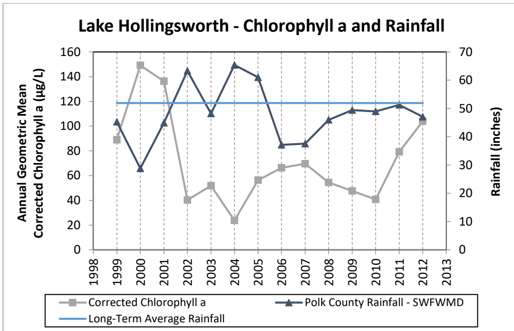
Figure 5.2 Lake Hollingsworth Chlorophyll a Annual Geometric Means and Annual Rainfall.
