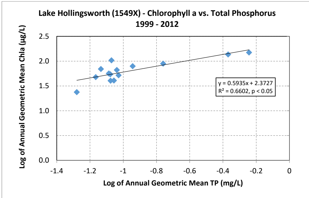
Figure 5.5 Relationship Between Annual Geometric Means of Chlorophyll a and Total Phosphorus in Lake Hollingsworth.
