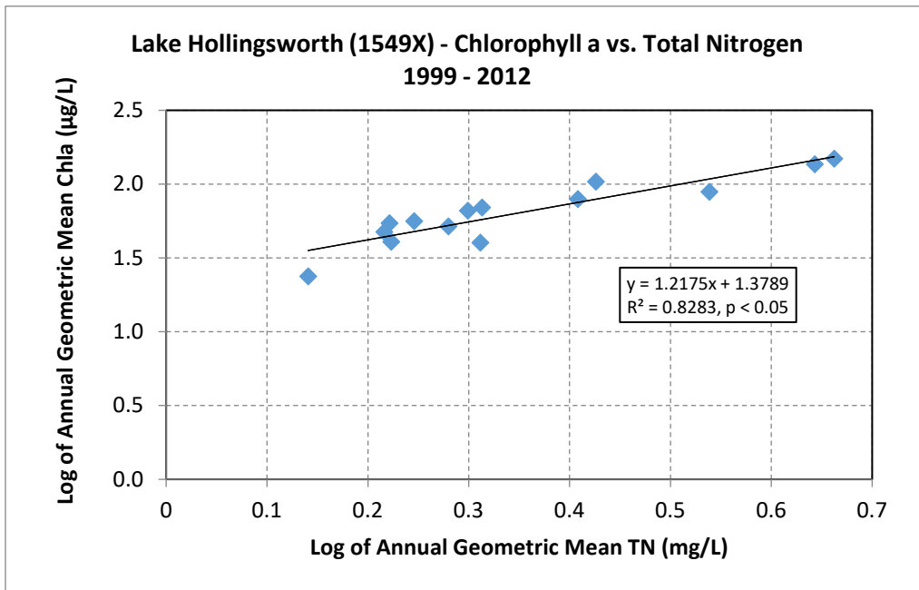
Figure 5.4 Relationship Between Annual Geometric Means of Chlorophyll a and Total Nitrogen in Lake Hollingsworth.
