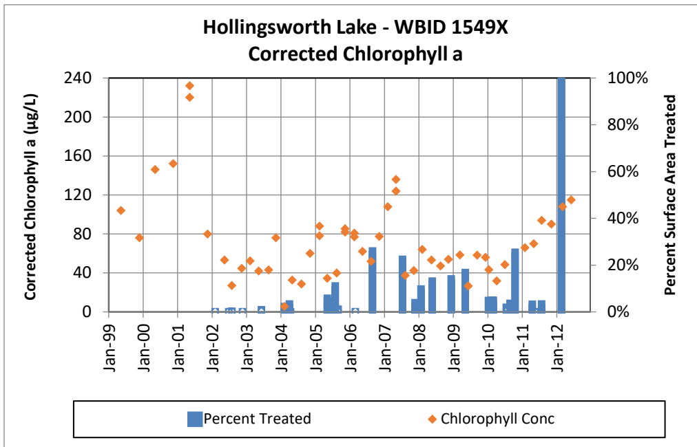
Figure 5.6 Lake Hollingsworth Chlorophyll a Results and Lake Area Treated for Invasive Aquatic Plant Growth.
