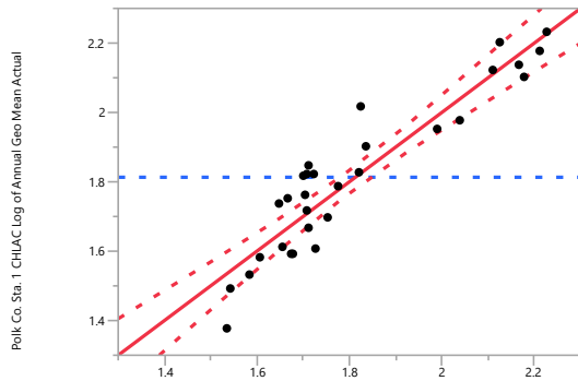
ta. 1 CHLAC Log of Annual Geo Mean Predicted P<.0001 RSq=0.87 RMSE=0.0859
