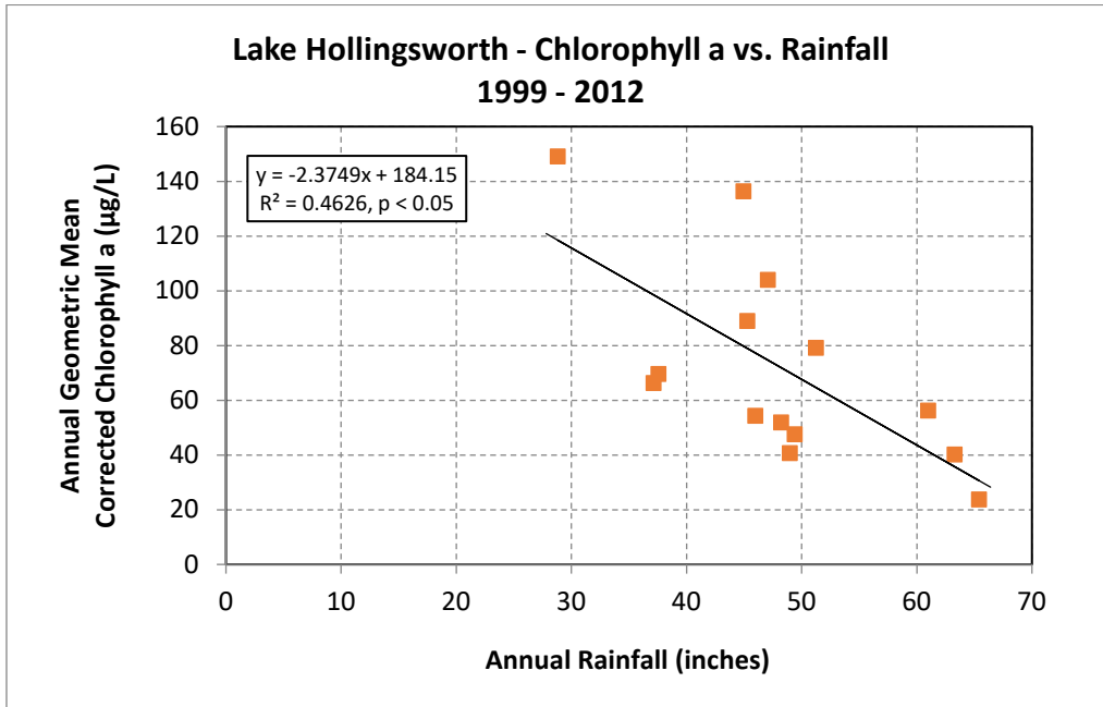
Figure 5.3 Relationship Between Lake Hollingsworth Chlorophyll a Annual Geometric Means and Annual Rainfall.
