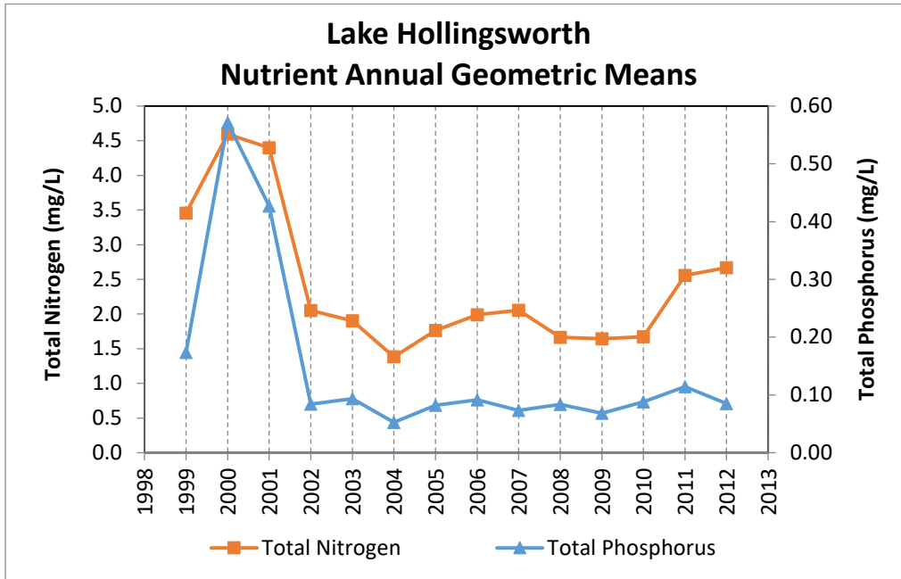
Figure 5.1 Total Nitrogen and Total Phosphorus Annual Geometric Means in Lake Hollingsworth.
