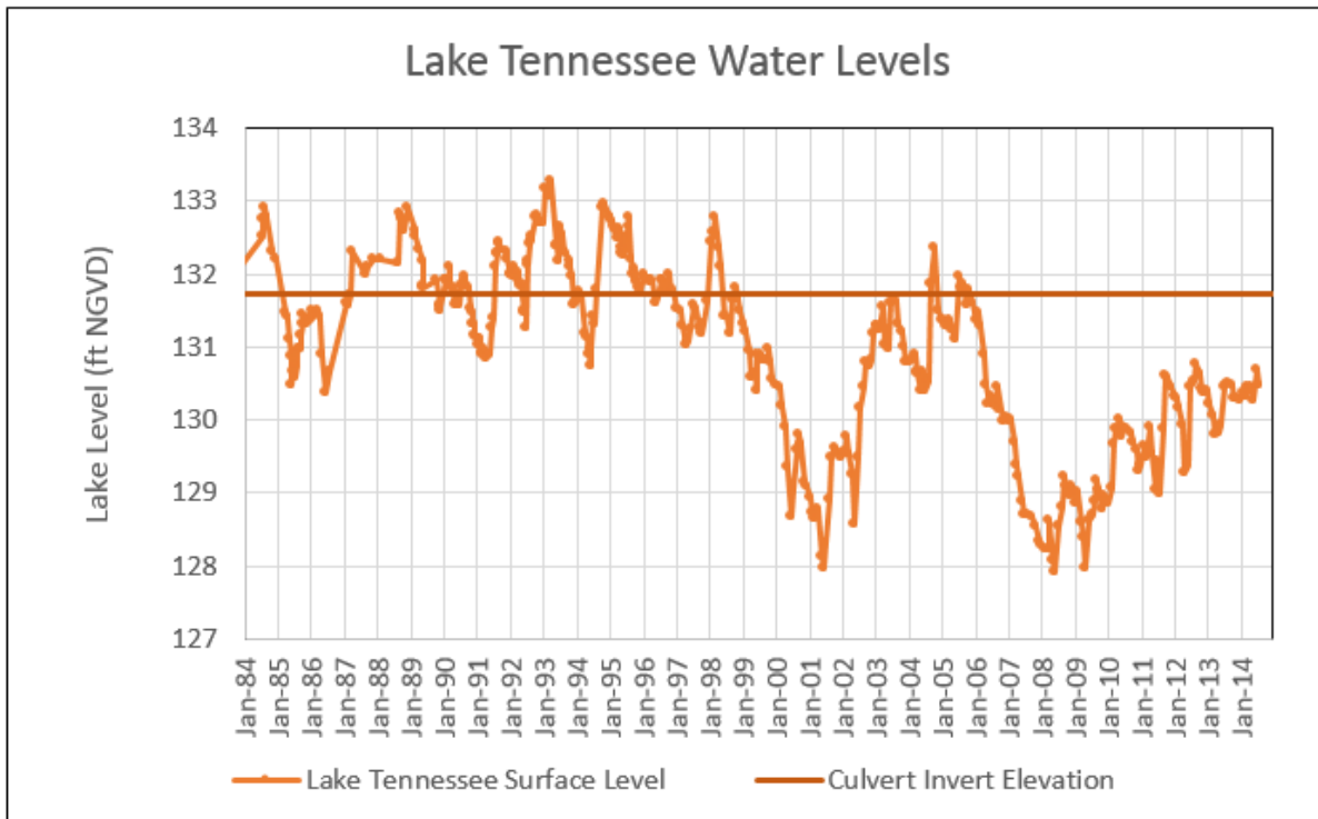
Figure 4.1. Lake Tennessee Surface Level in Relation to the Invert Elevation of the Outlet Pipes
