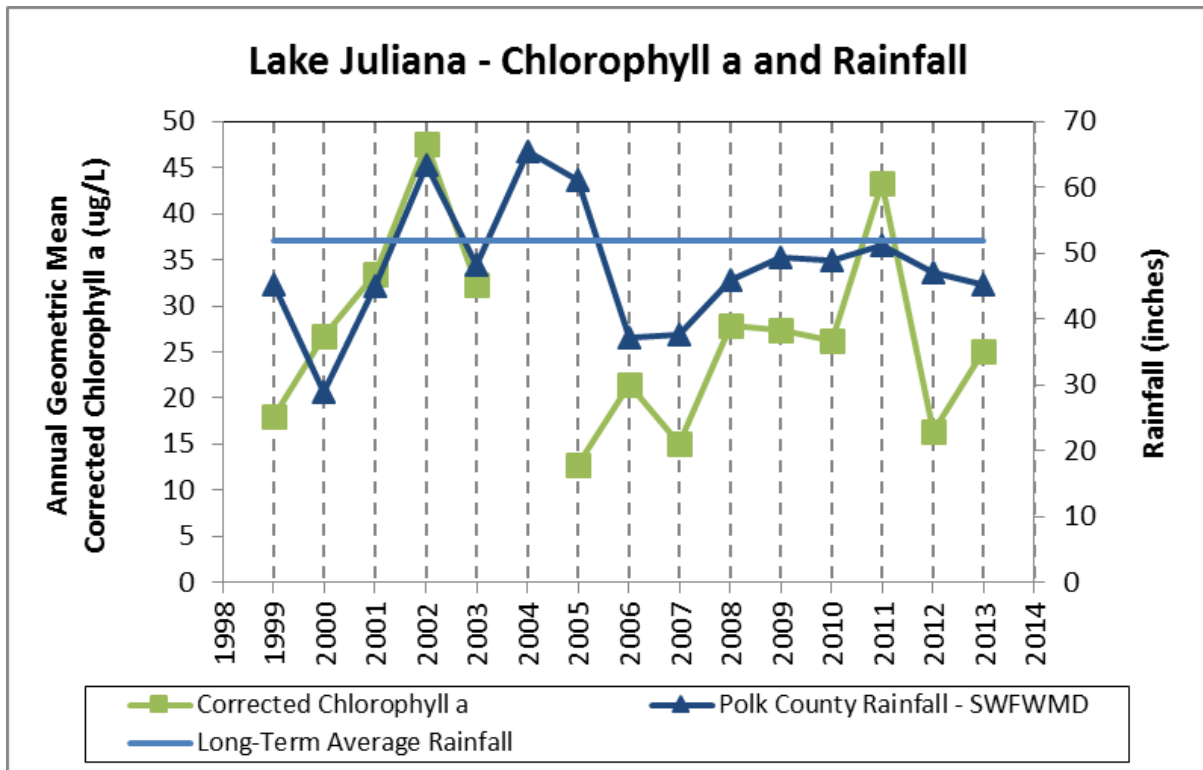
Figure 5.3. Lake Juliana Chlorophyll a AGMs, Based on Lake Center Results, and Annual Rainfall
