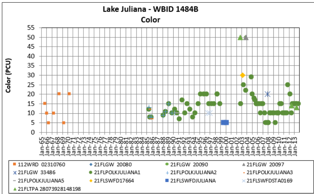
Figure B-4. Lake Juliana Color Results for Period of Record
