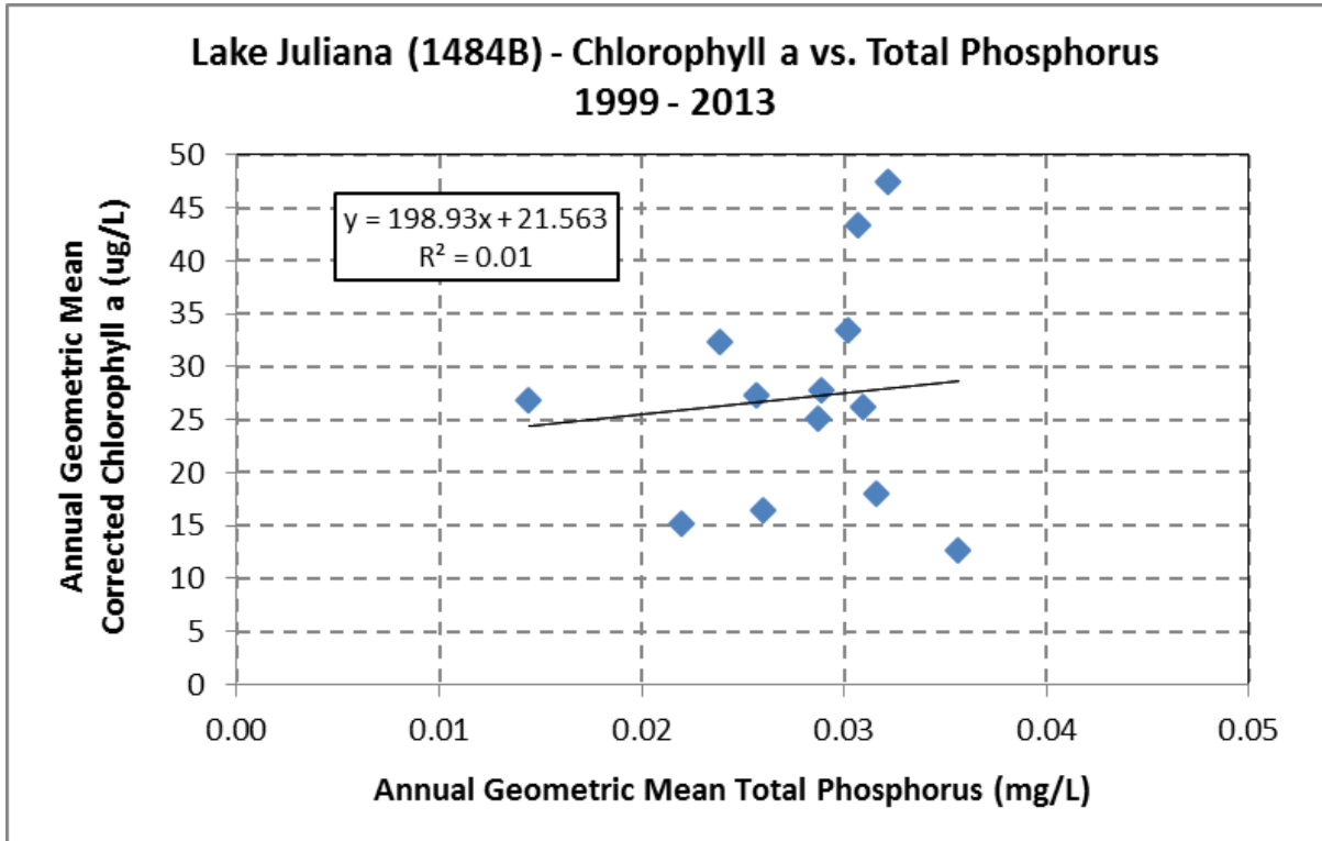
Figure 5.10. Relationship between AGMs of Chlorophyll a and TP in Lake Juliana
