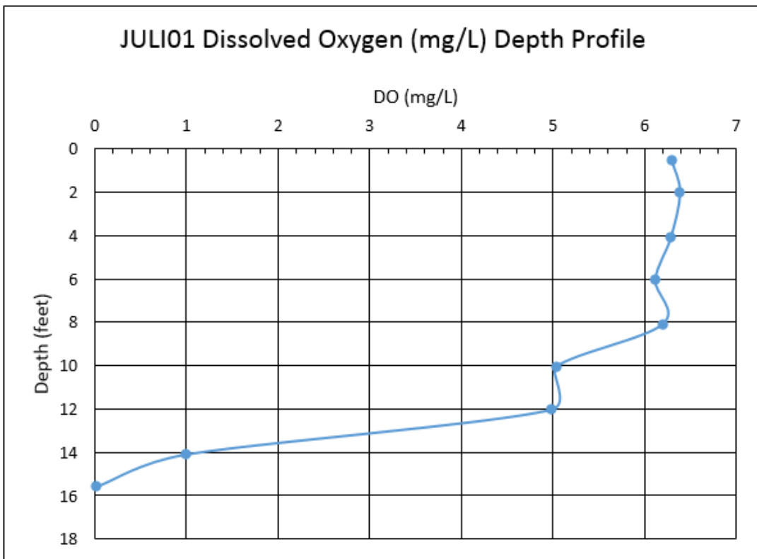
Figure D-1. Depth Profile for DO (mg/L) at JULI01
