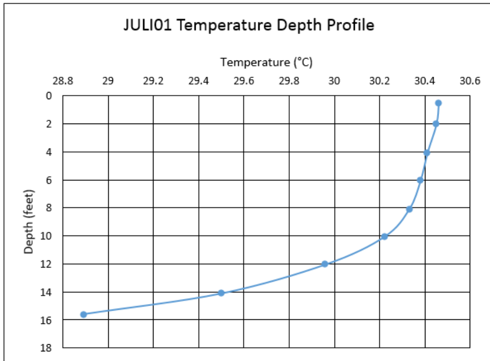
Figure D-4. Depth Profile for Temperature at JULI01
