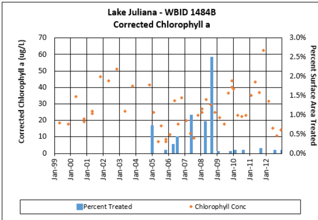
Figure 5.12. Lake Juliana Chlorophyll a Results and Lake Area Treated for Invasive Aquatic Plant Growth
