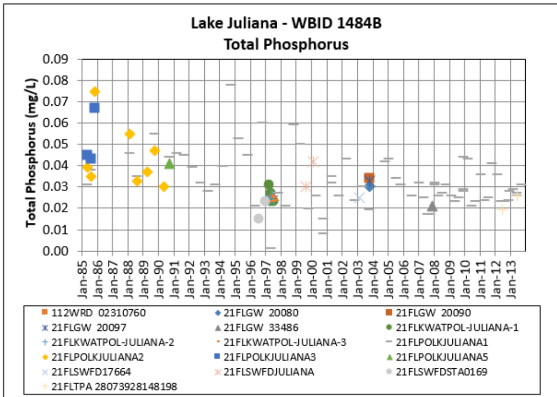
Figure B-3. Lake Juliana TP Results for Period of Record
