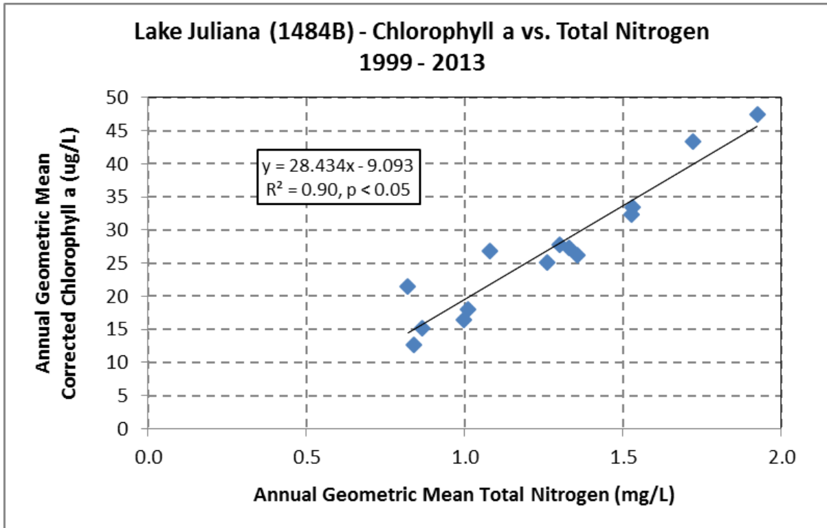
Figure 5.9. Relationship between AGMs of Chlorophyll a and TN in Lake Juliana
