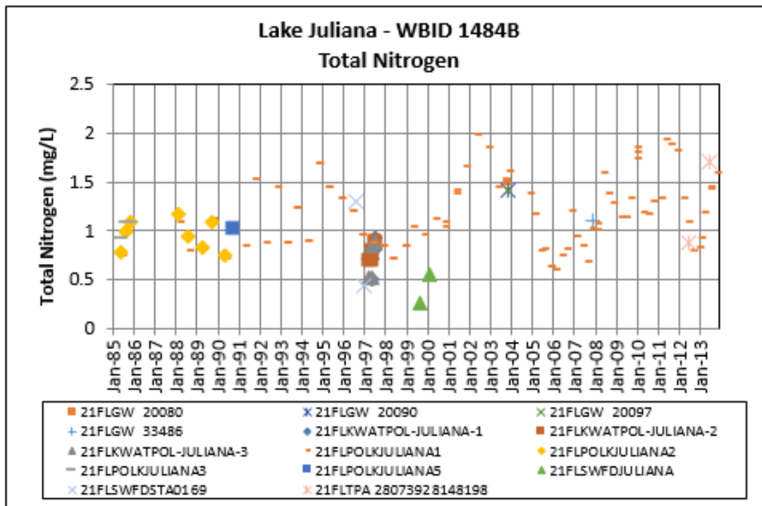
Figure B-2. Lake Juliana TN Results for Period of Record
