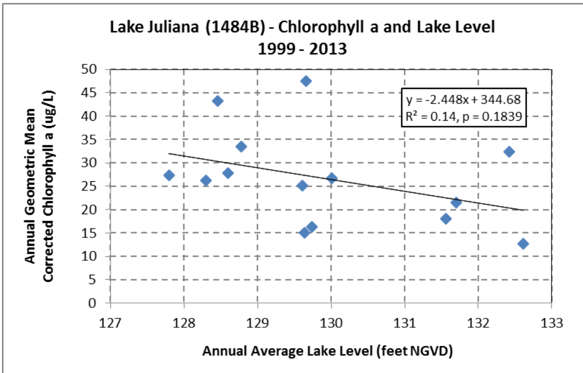
Figure 5.7. Relationship between Lake Juliana Chlorophyll a AGMs, Based on Lake Center Results, and Lake Level
