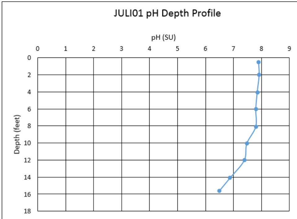
Figure D-2. Depth Profile for pH at JULI01
