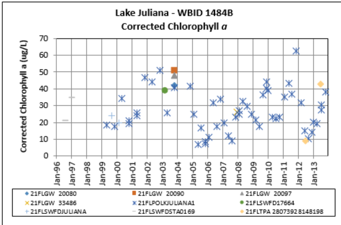
Figure B-1. Lake Juliana Corrected Chlorophyll a Results for Period of Record
