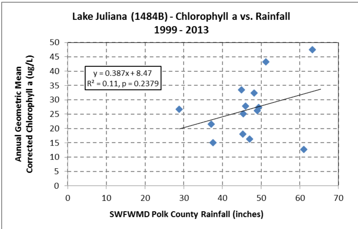
Figure 5.4. Relationship between Lake Juliana Chlorophyll a AGMs and Annual Rainfall
