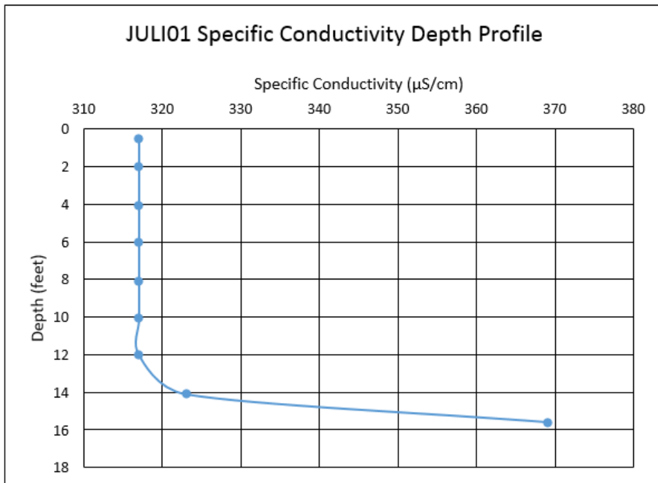
Figure D-3. Depth Profile for Specific Conductivity at JULI01
