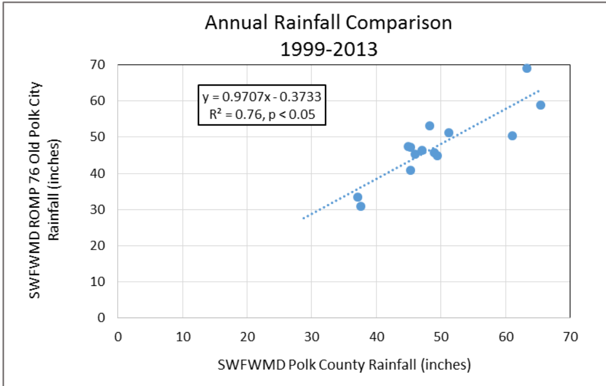
Figure 5.2. Comparison of SWFWMD Site-Specific and Countywide Rainfall Results
