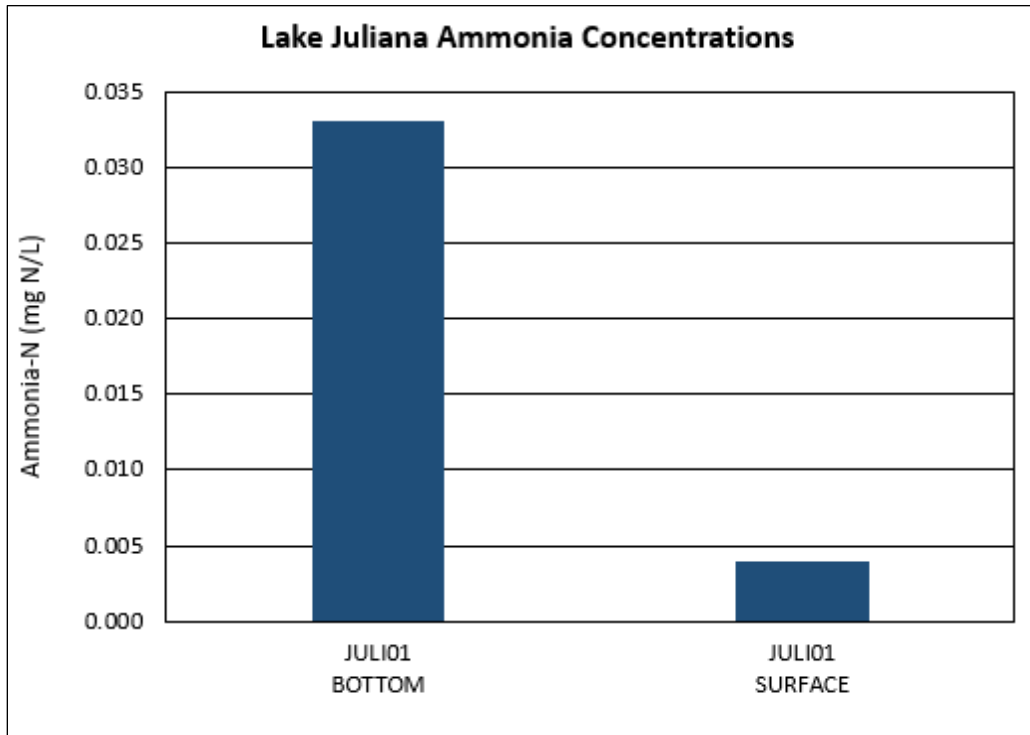
Figure 5.11. Lake Juliana Ammonia Concentrations Collected on August 5, 2014
