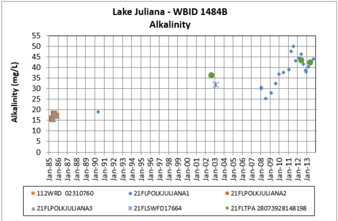
Figure B-5. Lake Juliana Alkalinity Results for Period of Record
