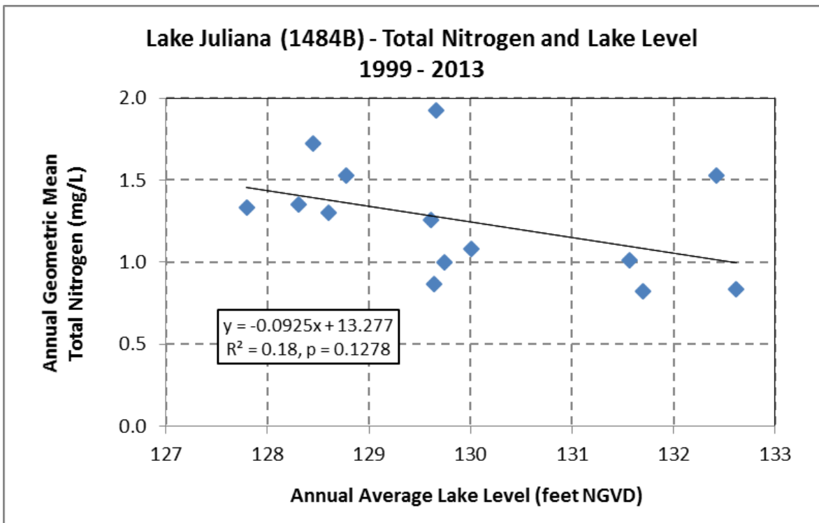
Figure 5.8. Relationship between Lake Juliana TN AGMs, Based on Lake Center Results, and Lake Level
