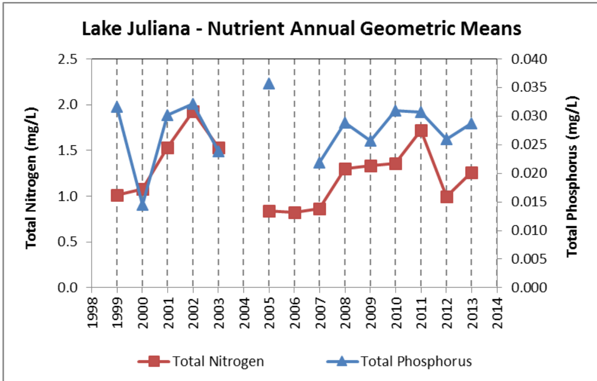
Figure 5.1. TN and TP AGMs in Lake Juliana, Based on Lake Center Results
