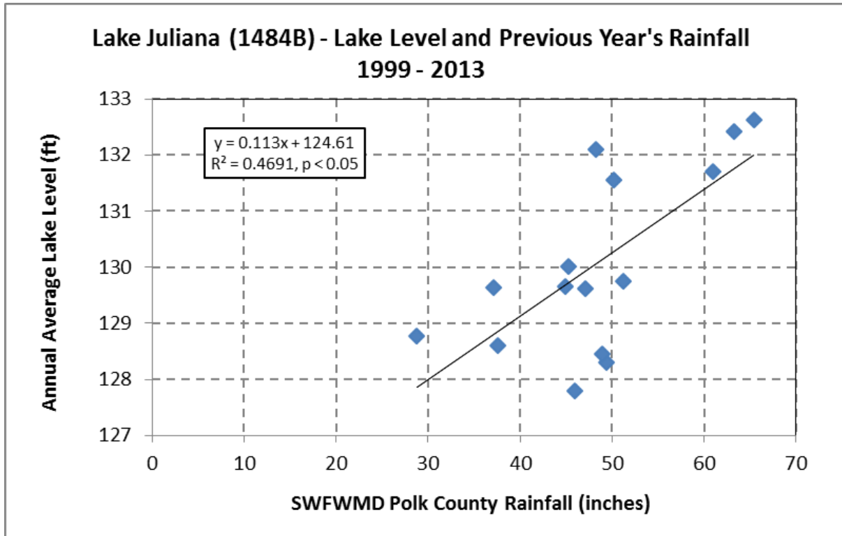
Figure 5.5. Relationship between Lake Juliana Water Level and Previous Year’s Rainfall
